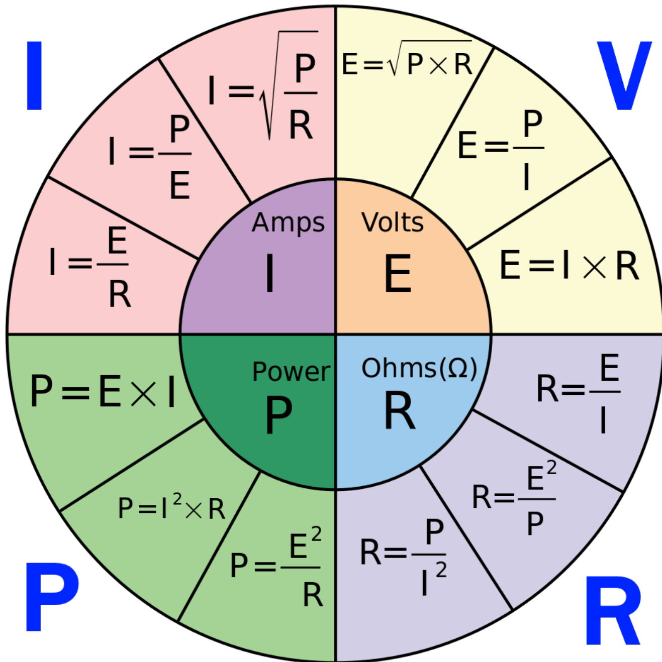
Power, Voltage, Current & Resistance Calculator
